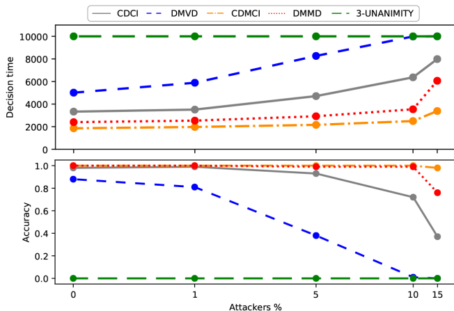
Fig. 1. Effect of contrarians on the decision dynamics of a swarm of S = 100 simulated robots with n = 6 options and decision difficulty \kappa = q_L/q_H = 0.8 . The points show the average of 100 multiagent simulations. The top panel shows the slow down effect of contrarians that increase the decision time. High decision time hinders the accuracy of the swarm (bottom panel). The most resilient method is the CDMCI (orange dash-dotted line). Comparing CDCI (gray full line) and DMVD (blue short-dashed line), we can appreciate a resiliency increase for the method that relies on the cross-inhibition model rather than the direct switch model. Comparing DMVD (blue short-dashed line) and DMMD (red dotted line), we can appreciate a resiliency increase for the method that relies on the majority-rule rather than the random selection (voter model).
